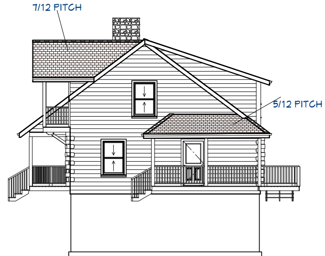
Exterior Elevation Right
