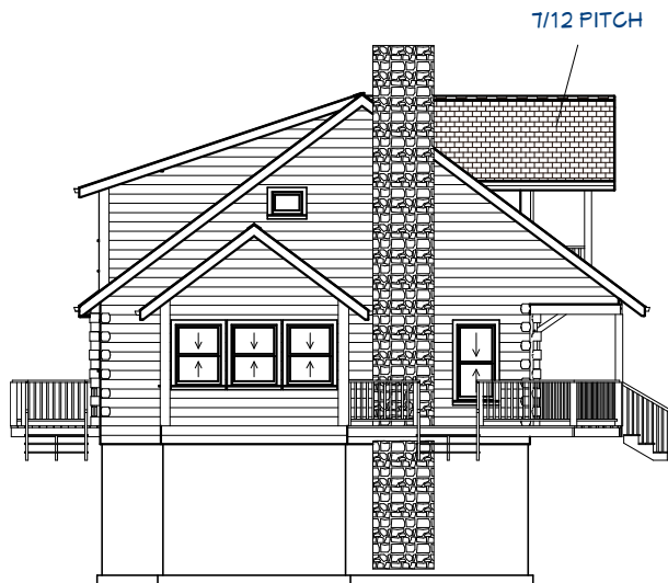
Exterior Elevation Left
