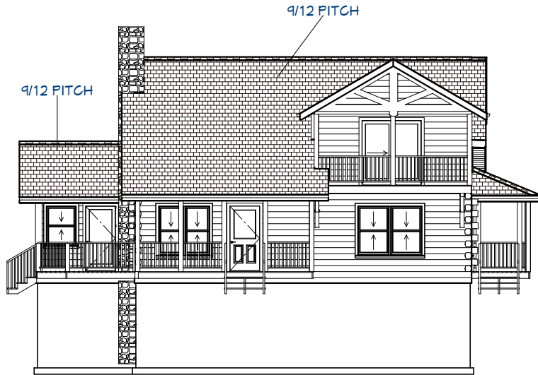
Exterior Elevation Front
