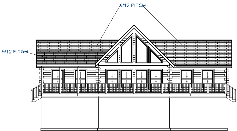
Exterior Elevation Front
