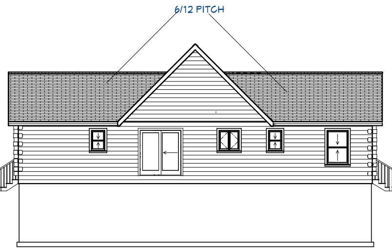
Exterior Elevation Back
