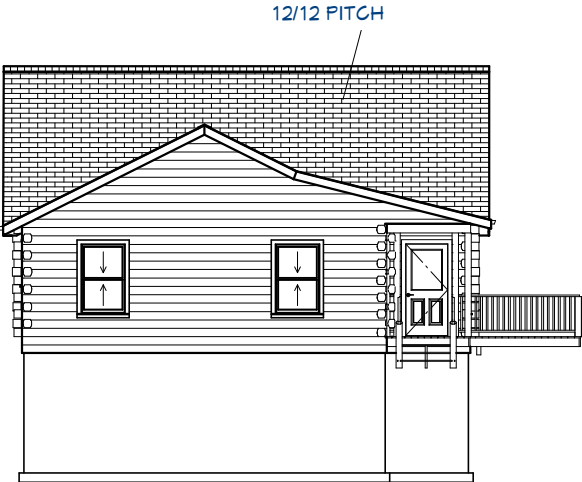
Exterior Elevation Left
