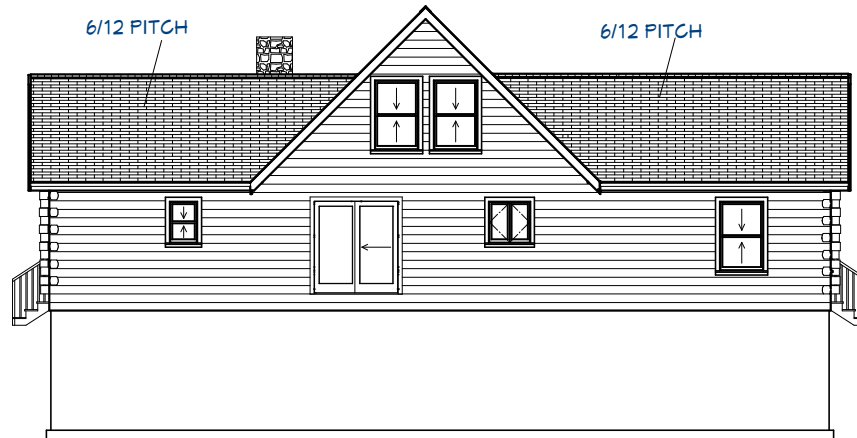
Exterior Elevation Back
