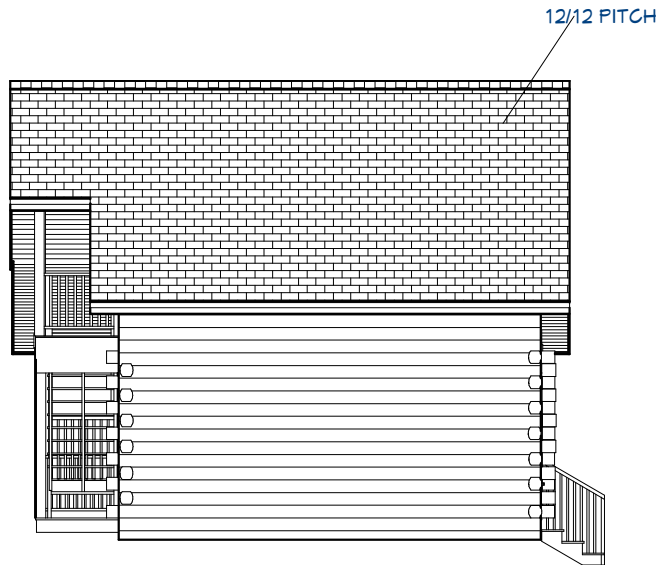
Exterior Elevation Left
