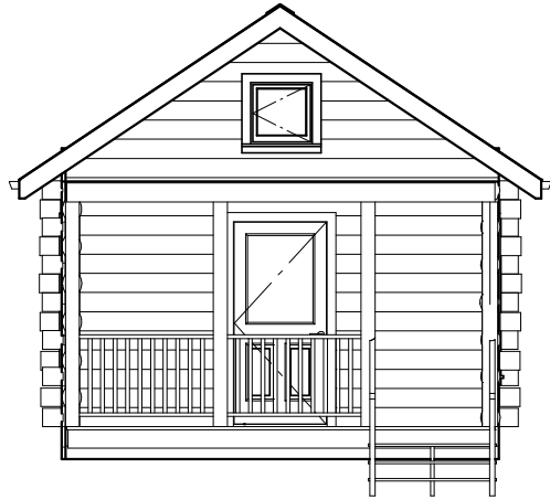
Exterior Elevation Front
