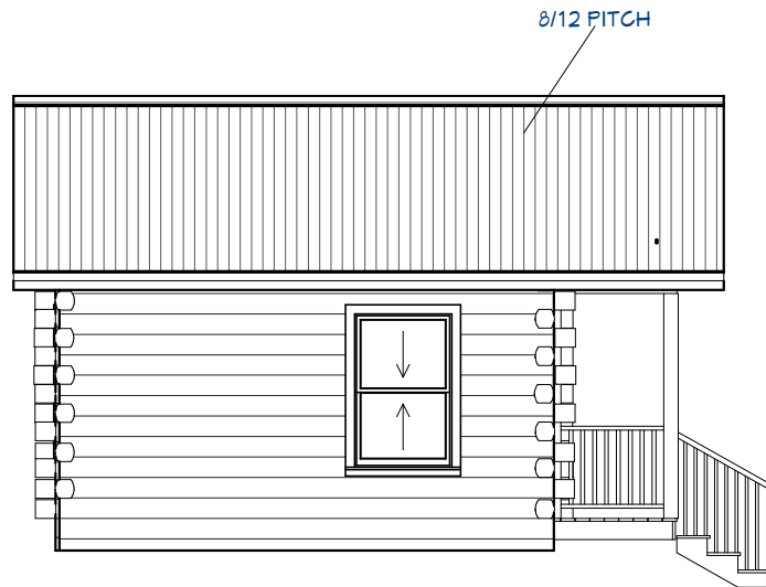
Exterior Elevation Left
