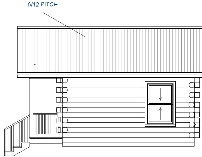
Exterior Elevation Right
