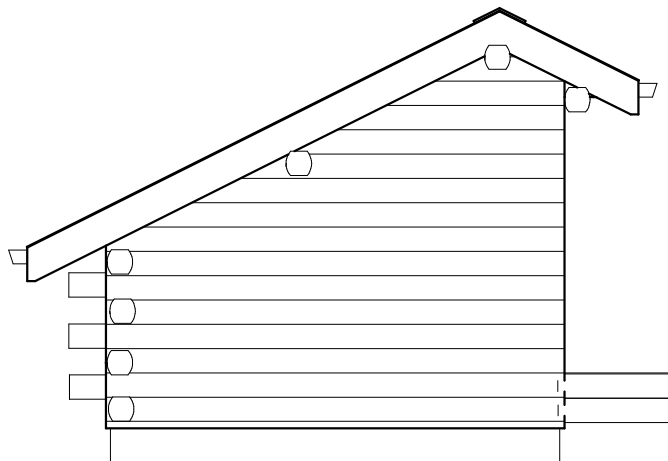
Exterior Elevation Left
