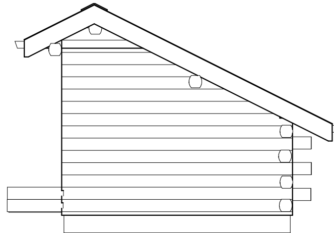
Exterior Elevation Right
