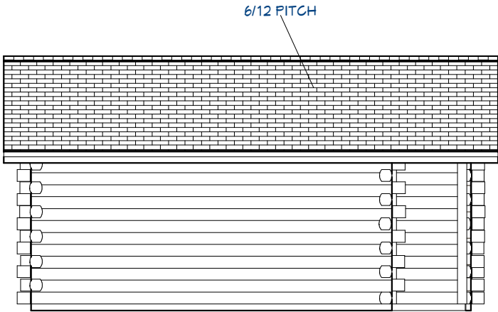
Exterior Elevation Left
