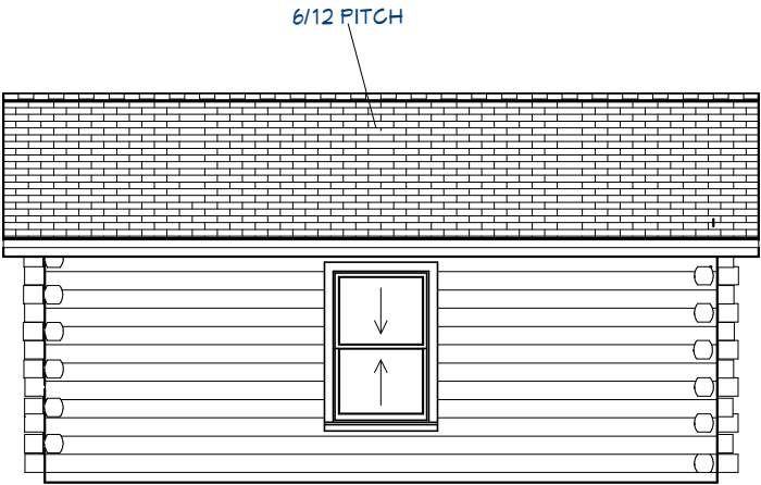
Exterior Elevation Right
