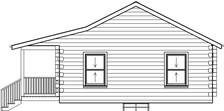
Exterior Elevation Right
