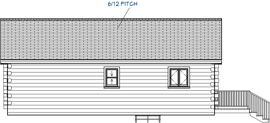
Exterior Elevation Back
