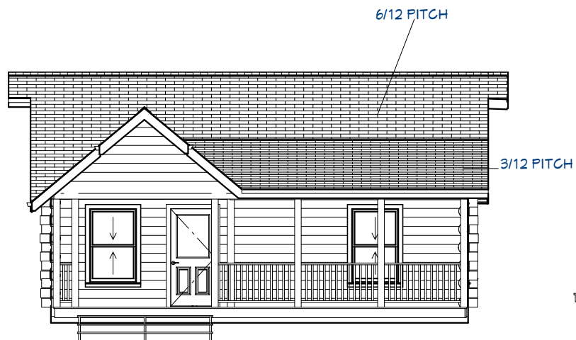
Exterior Elevation Front
