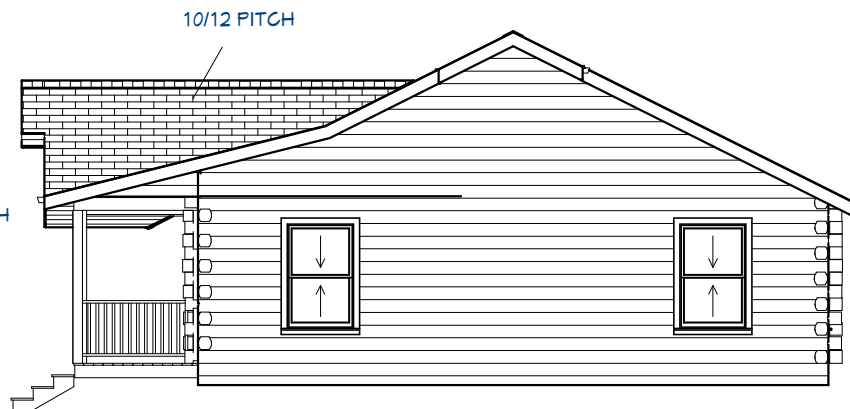
Exterior Elevation Right
