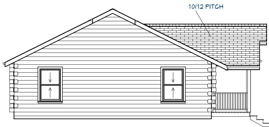
Exterior Elevation Left
