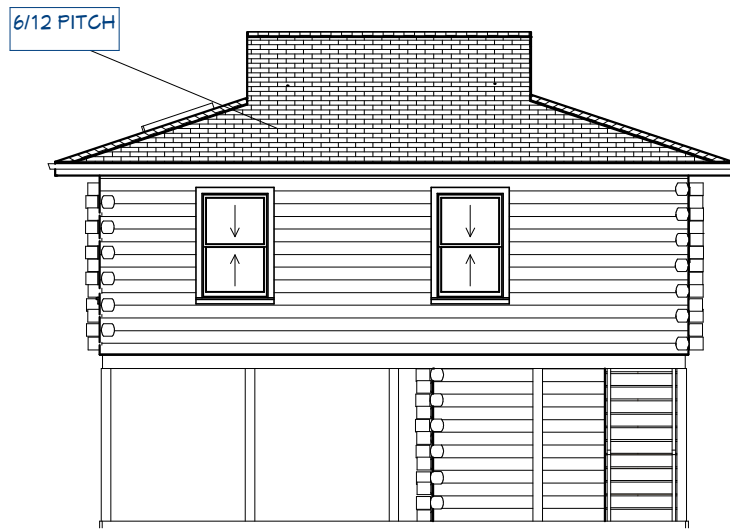
Exterior Elevation Right
