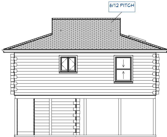
Exterior Elevation Left
