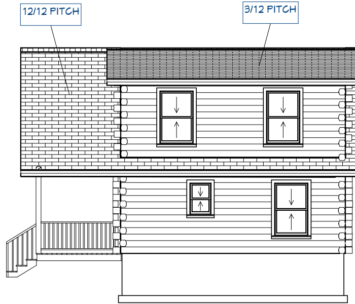
Exterior Elevation Right
