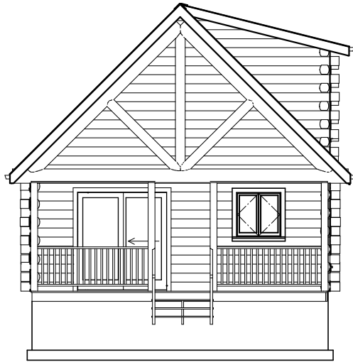
Exterior Elevation Front
