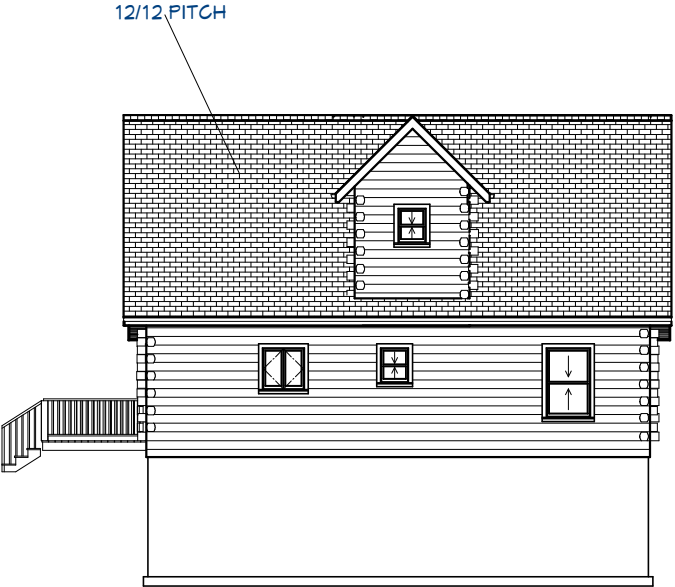
Exterior Elevation Right
