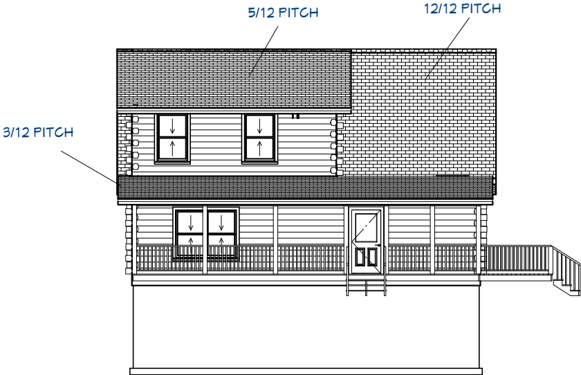
Exterior Elevation Left
