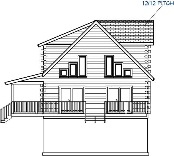
Exterior Elevation Front
