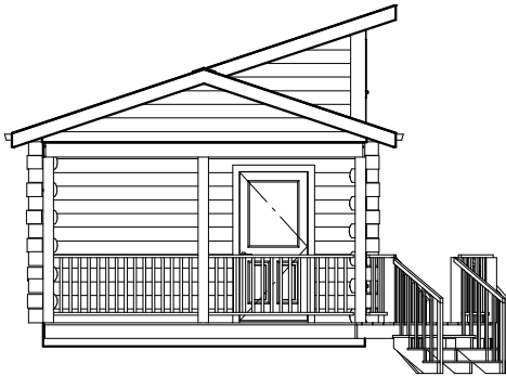
Exterior Elevation Left
