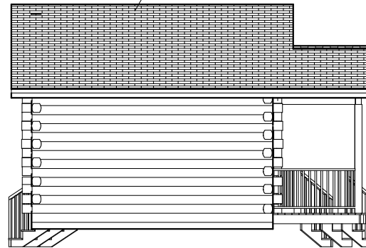
Exterior Elevation Back
