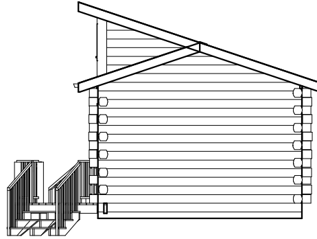
Exterior Elevation Right
