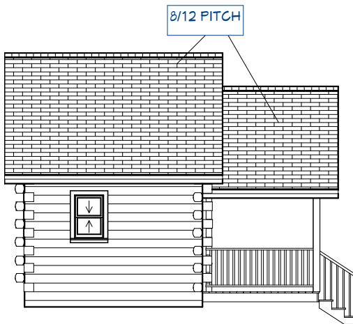
Exterior Elevation Left
