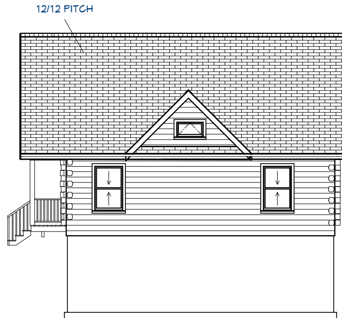
Exterior Elevation Right
