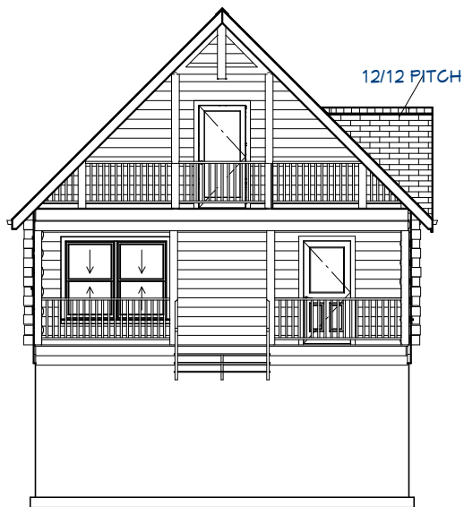
Exterior Elevation Front
