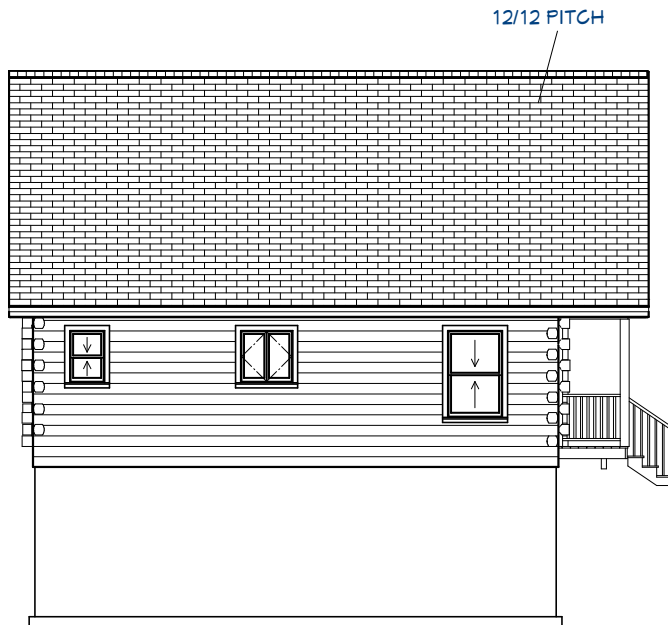
Exterior Elevation Left
