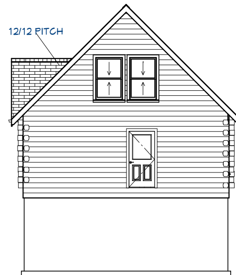
Exterior Elevation Back
