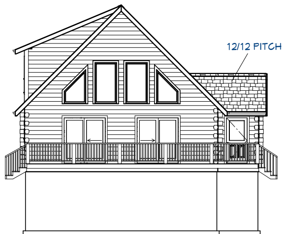
Exterior Elevation Front
