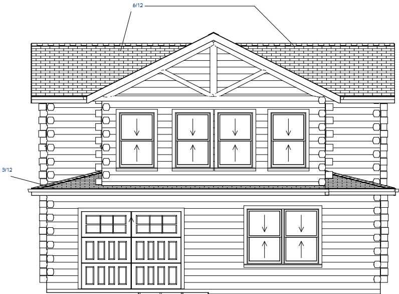
Exterior Elevation Front
