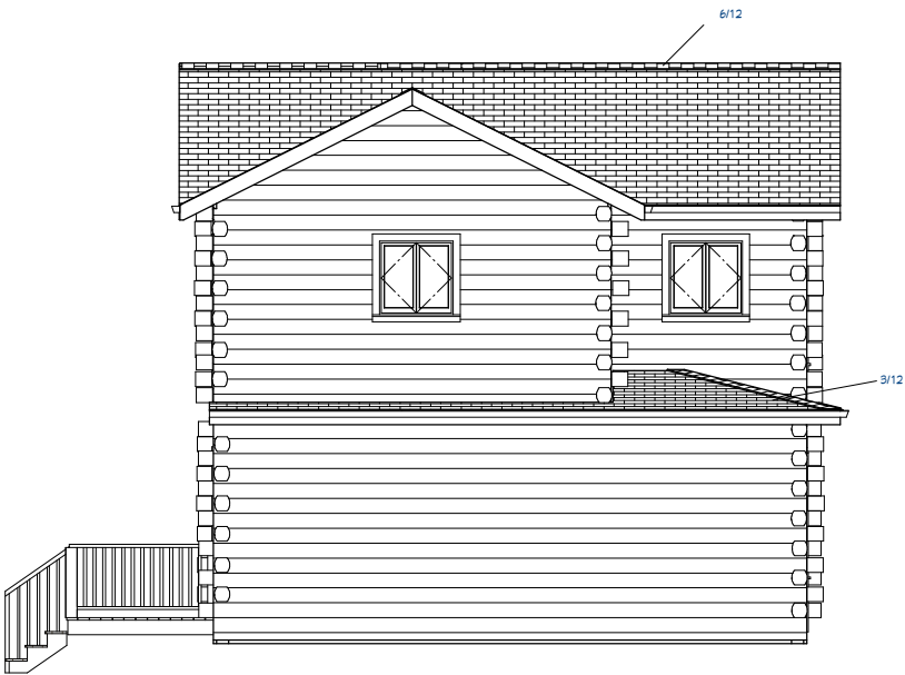
Exterior Elevation Front
