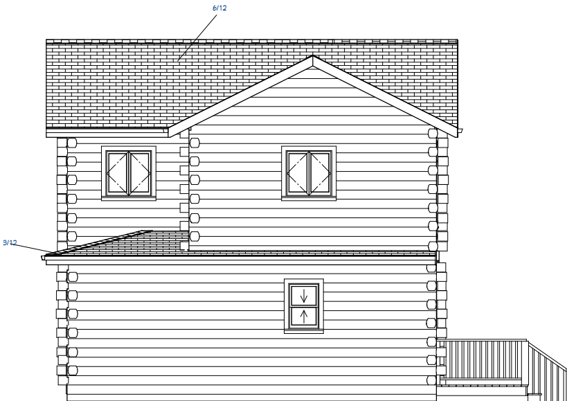
Exterior Elevation Right
