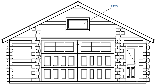
Exterior Elevation Front
