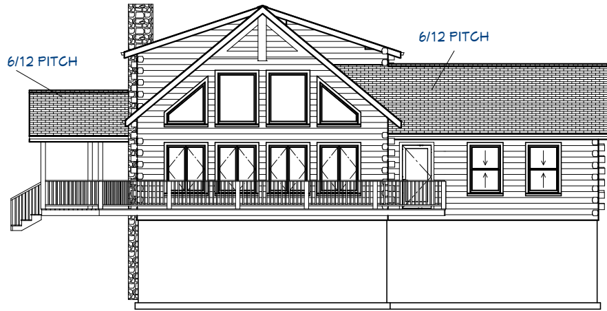
Exterior Elevation Front
