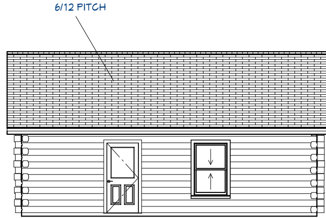
Exterior Elevation Right
